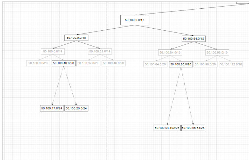
Virtual Blocks vs Real Blocks example diagram
